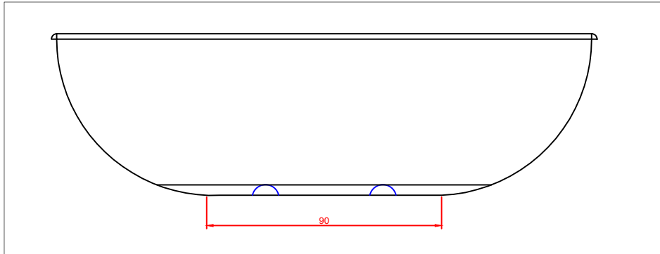
SIDE VIEW 2 (DESIGN 1)
