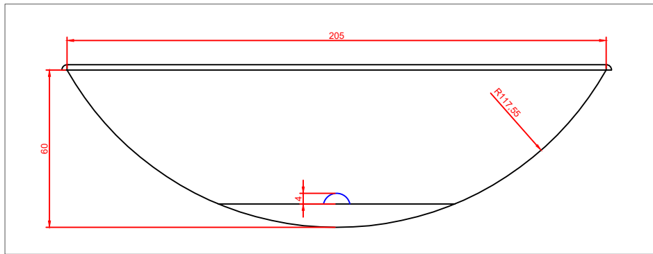
SIDE VIEW (DESIGN 2)
